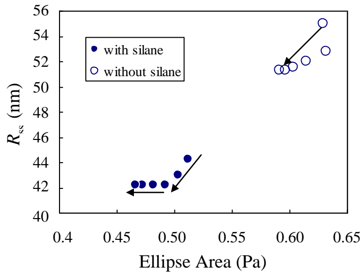
Fig.6 R_{ss} as a Function of Ellipse Area at 200% Shear Strain Amplitude
